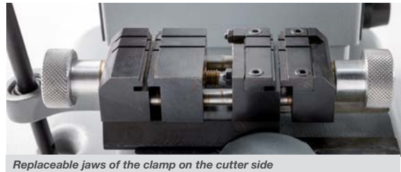
Replaceable jaws of the clamp on the cutter side
